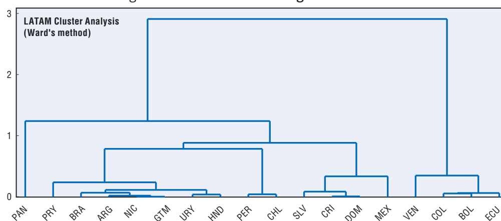
Figure 5.A1.1. Cluster dendrogram
