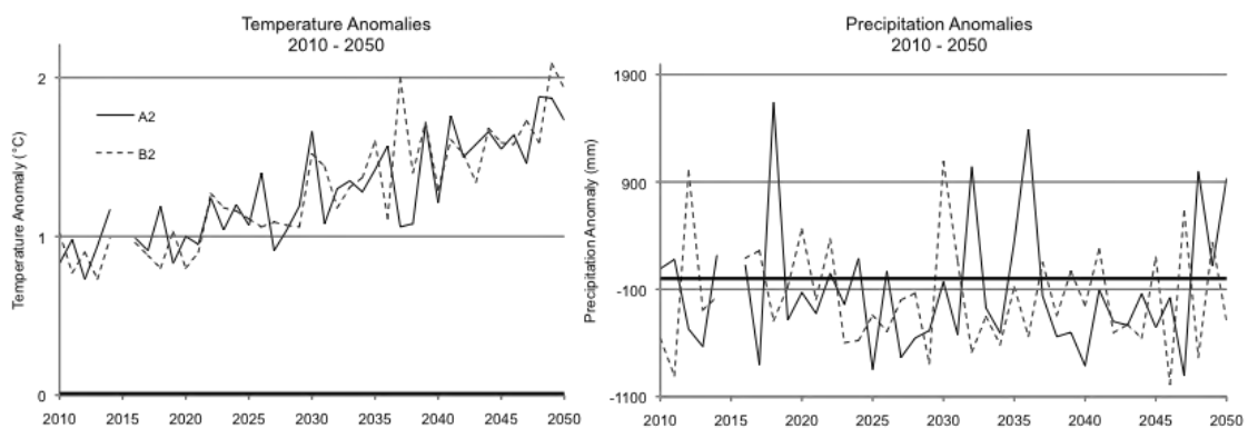
Figure 10: ECHAM4 down-scaled A2 and B2 Precipitation and Temperature Anomalies 2010-2050
