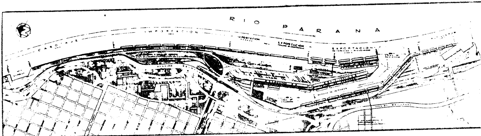
FUTURE LAY-OUT OF ROSARIO PORT
